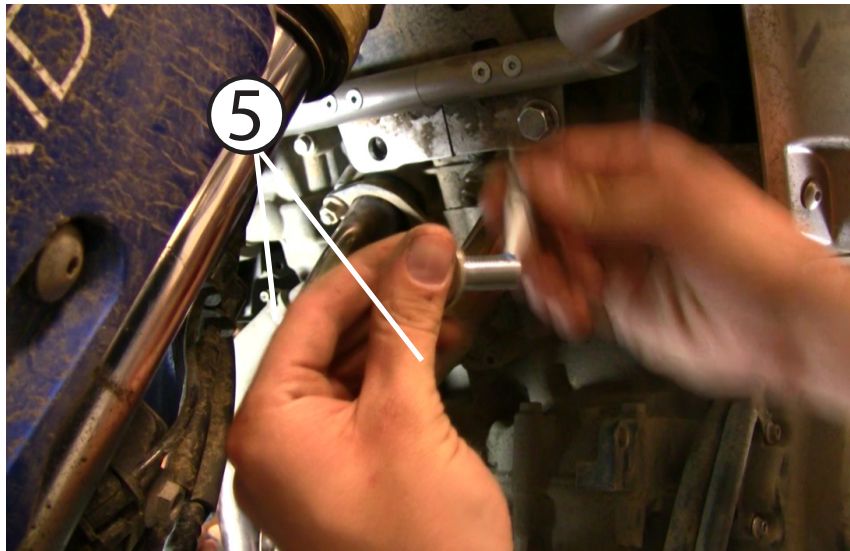
⑤ After applying a drop of thread locker to the end of the provided M12 fasteners, use a 19mm socket to install these bolts to the front center plates. Do not tighten these all the way down just yet.
