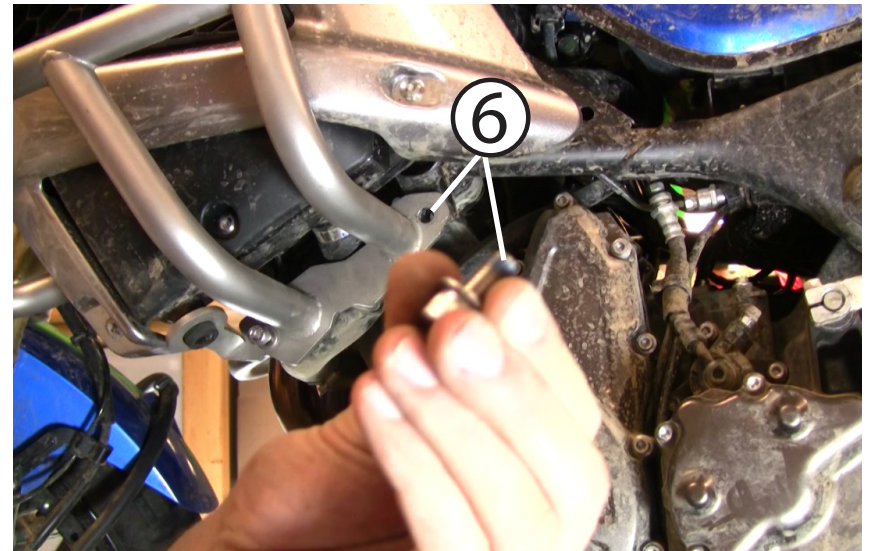
⑥ After applying a drop of thread locker to the end of the provided M8 fasteners, use a 6mm allen tool to install these bolts to the left and right mount brackets. Do not tighten these all the way down just yet. (be sure to do both the left and right mount brackets!)(long screw goes in left front)
