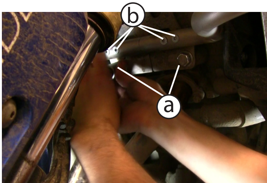
⑦ (a) Using a 19mm socket, tighten these two provided fasteners to 75nm of torque. (b) Using a 4mm allen tool with a torque wrench, torque these fasteners to 8nm.
