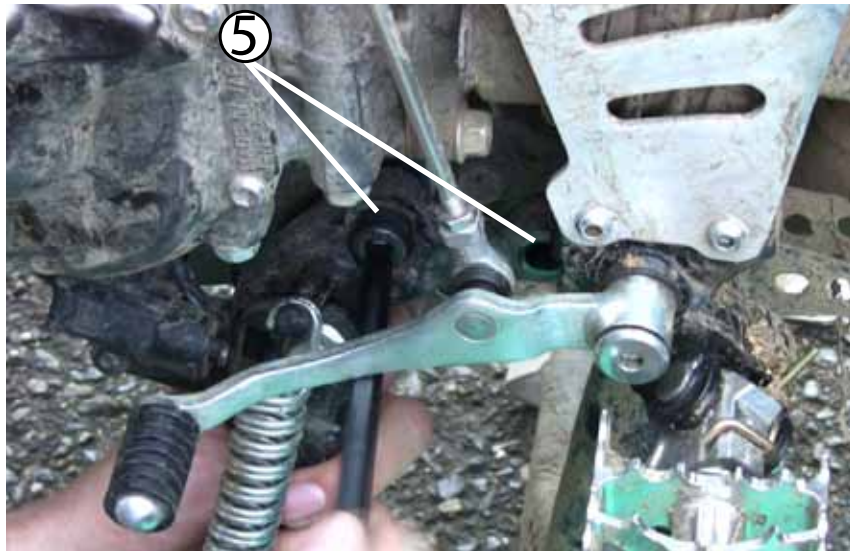
⑤ Using an 8mm allen tool, remove these (2) OEM fasteners. Keep them around, you will not be reusing them. When you remove the side stand, a spacer will drop out, you will not be reusing this.
