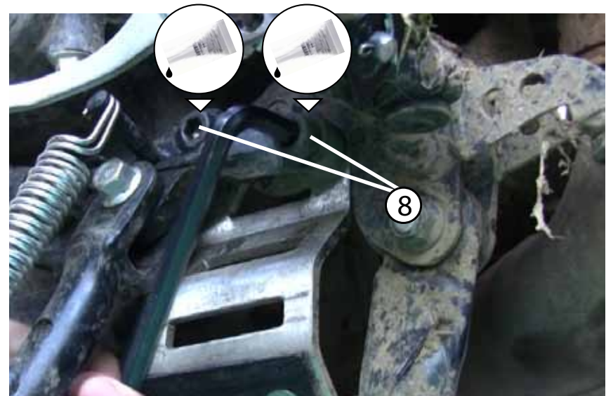
⑧ Put the sidestand back up to its mount holes. You no longer need the spacer that came out when you removed the OEM bolts. Apply thread locker, then using an 8mm allen tool, insert and tighten these (2) provided M10 x 40 bolts a few turns. Do not tighten all the way down yet.
