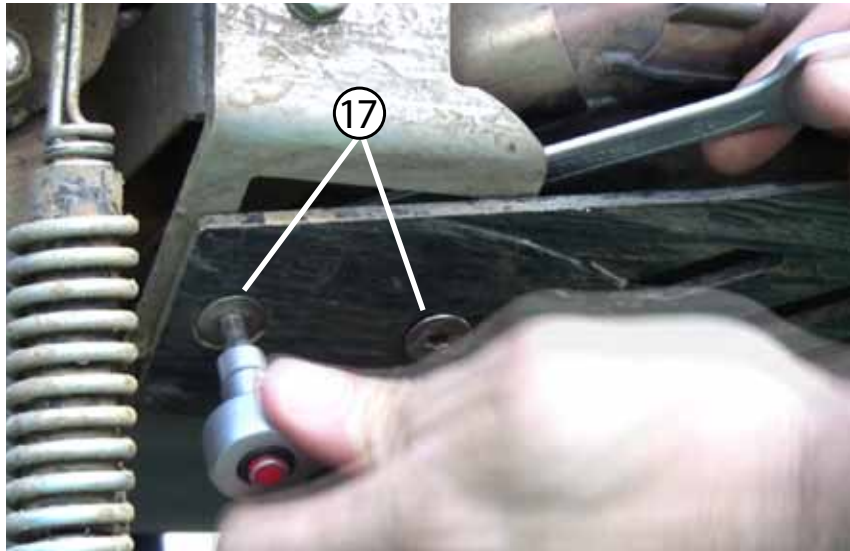
17 On the right side rear, using a 5mm allen tool and a 13mm wrench, tighten these two fasteners down.
