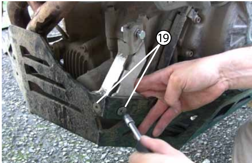
19 Using a 5mm allen tool and a 13mm wrench, tighten these two fasteners down.
