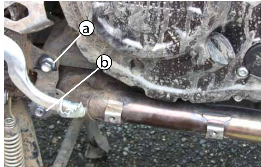
⑥ (a) Using a 15mm socket remove this fastener. (b) Using a 13mm socket remove this OEM fastener. You won't be reusing either of these fasteners.
