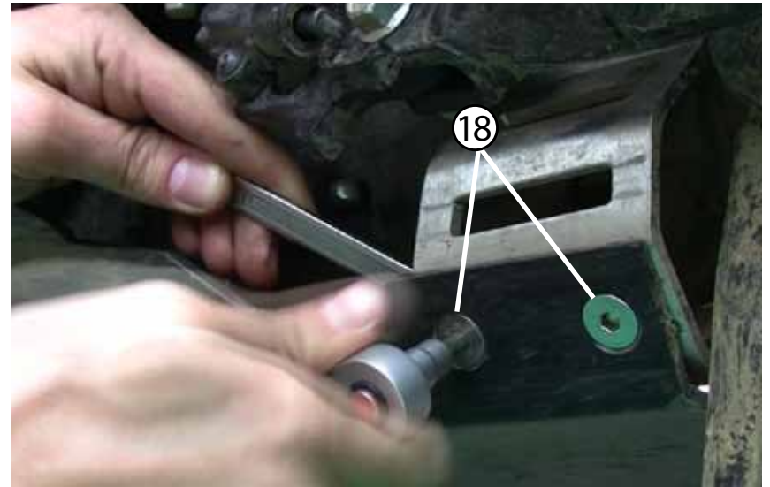
18 On the left side rear, use the 5mm allen tool and 13mm wrench to finish tightening these two fasteners.
