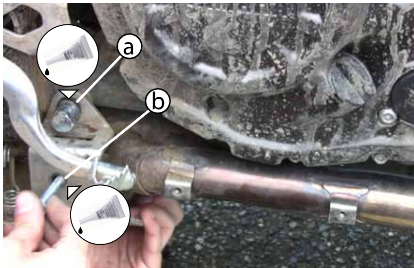
⑦ Hold rear mount bracket as shown and: (a) After applying thread locker to both fasteners, use a 17mm socket to start the M10 x 105 fastener and washer. (b) Use a 13mm socket, start the M8 x 45 fastener and washer. Do not tighten these all the way down yet.
