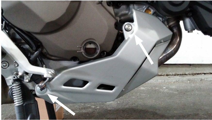
① Remove right side attachments. 4mm and 5mm allen wrenches.
