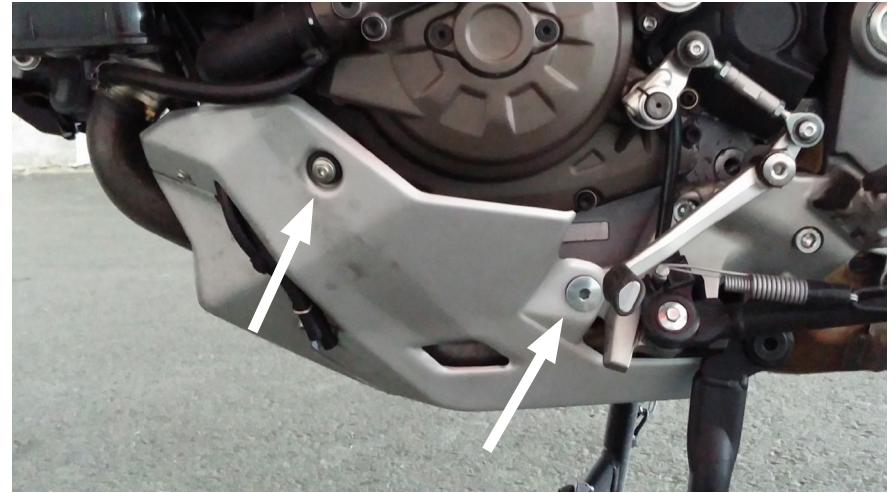
② Remove left side attachments. 4mm and 5mm allen wrenches.
